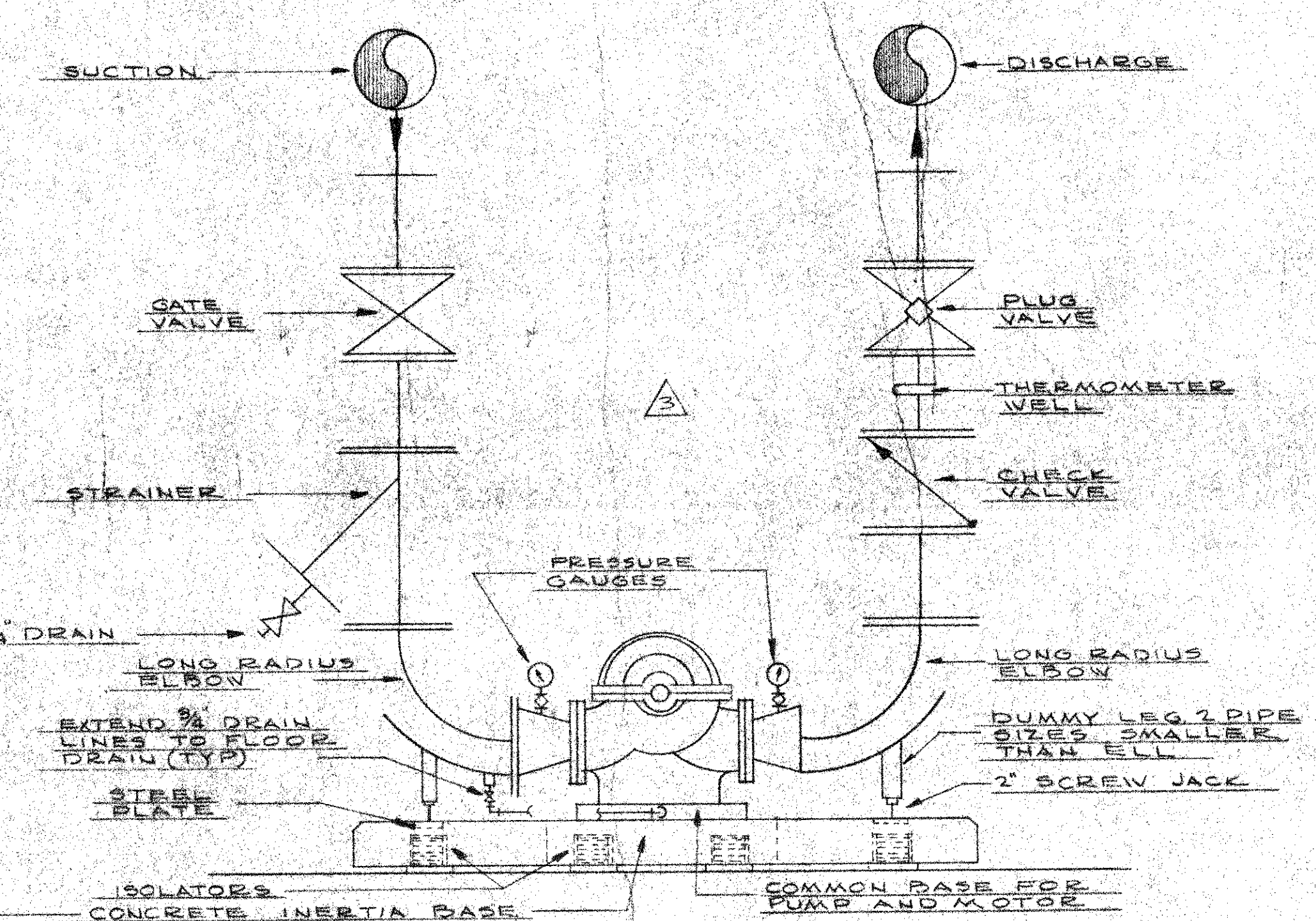
TYPICAL DOUBLE SUCTION CENTRIFUGAL PUMP PIPING DIAGRAM NO SCALE
