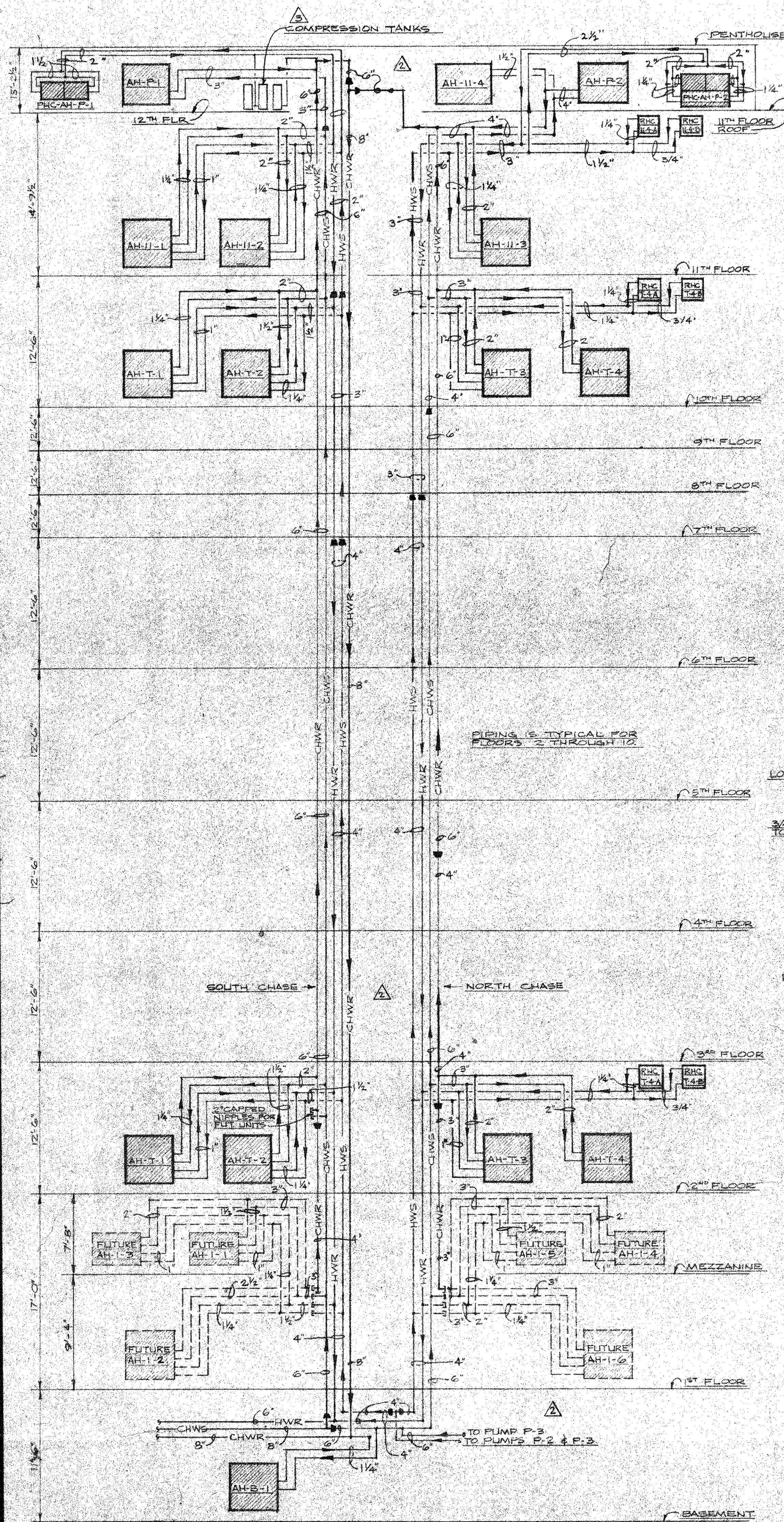
PIPING RISER DIAGRAM NO SCALE
