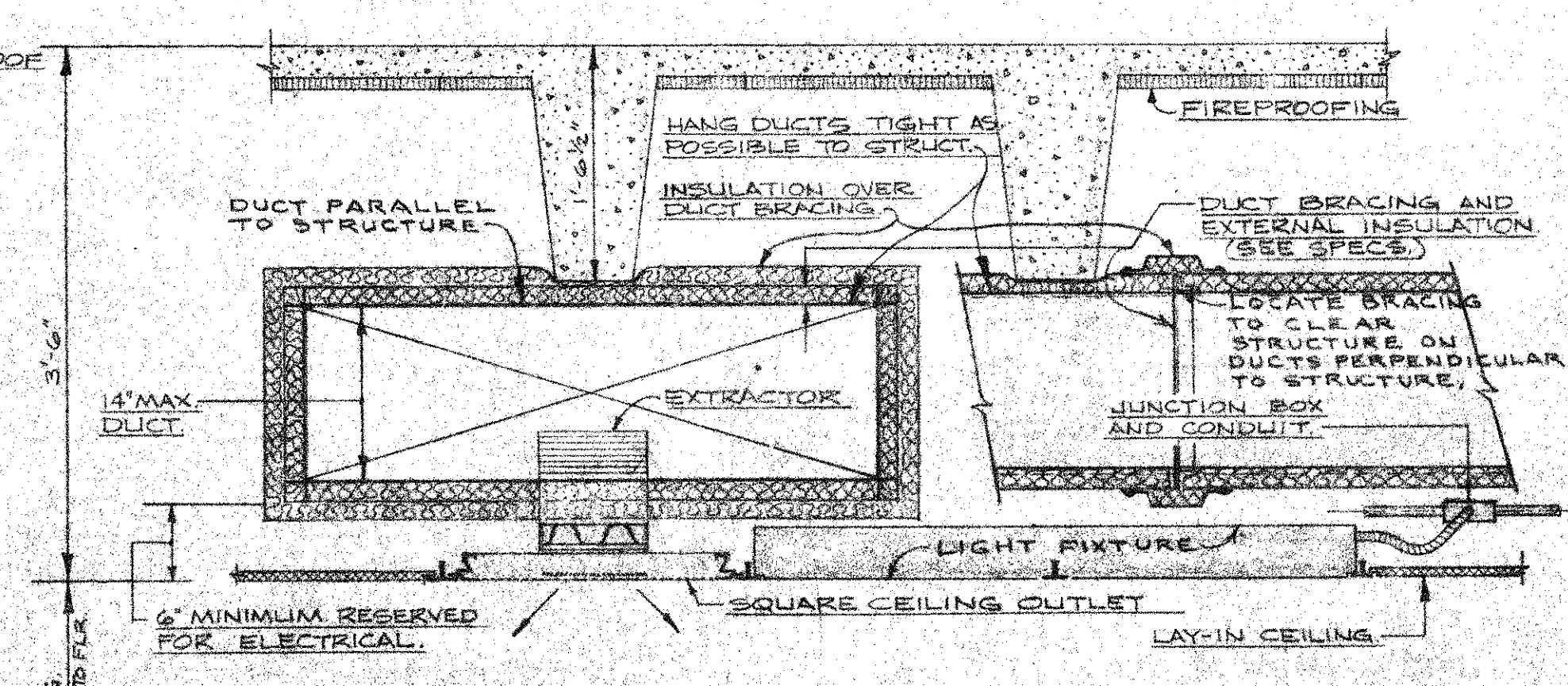
CRITICAL CONNECTION TO OUTLET UNDER TRUNK DUCT - DETAIL SCALE: 1" = 1'-0" NOTE LIMITATION ON CEILING OUTLET HEIGHT.
