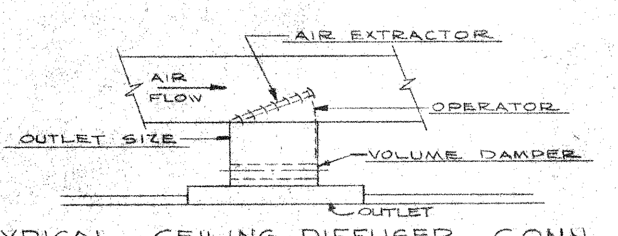
TYPICAL CEILING DIFFUSER CONN. DETAIL BELOW TRUNK DUCT NO SCALE
