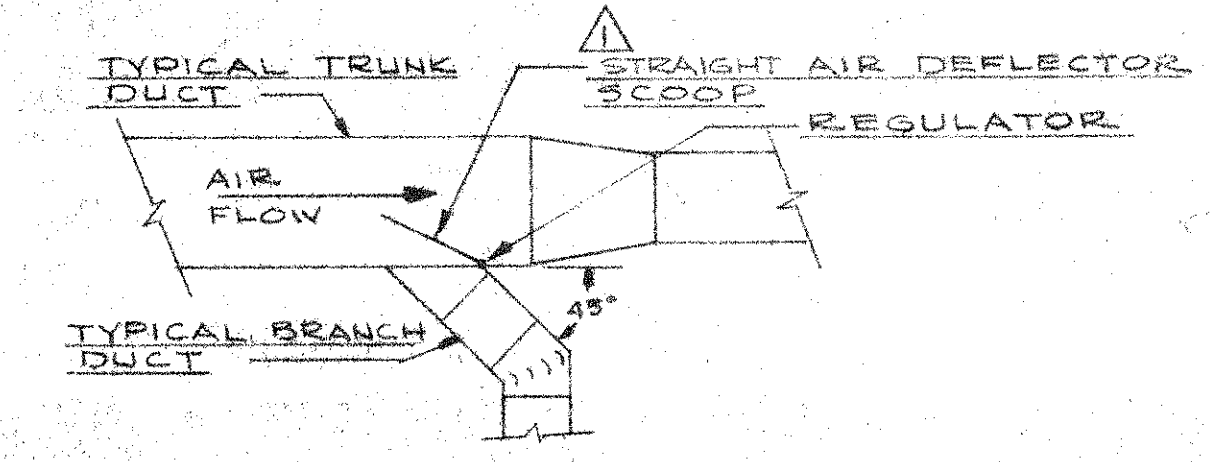
TYPICAL TRUNK DUCT TAKE-OFF DETAIL NO SCALE
