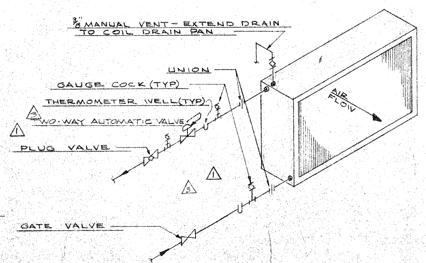
TYPICAL CHILLED WATER COIL, PREHEAT COIL, REHEAT COIL, & DOMESTIC WATER HEAT EXCHANGER PIPING DIAGRAM NO SCALE
