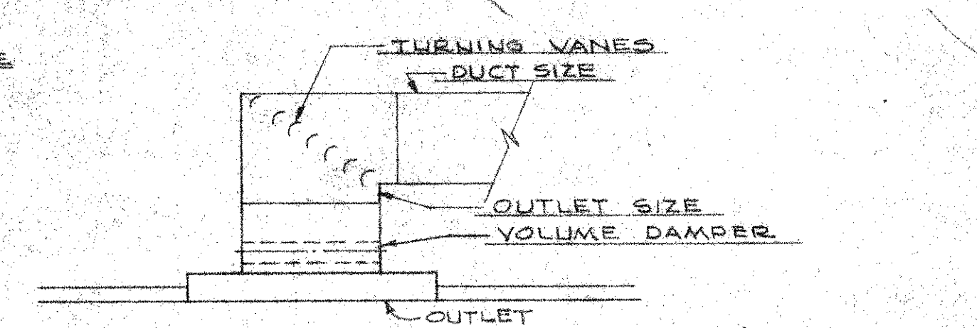
TYPICAL CEILING DIFFUSER CONN. DETAIL AT END OF DUCT NO SCALE
