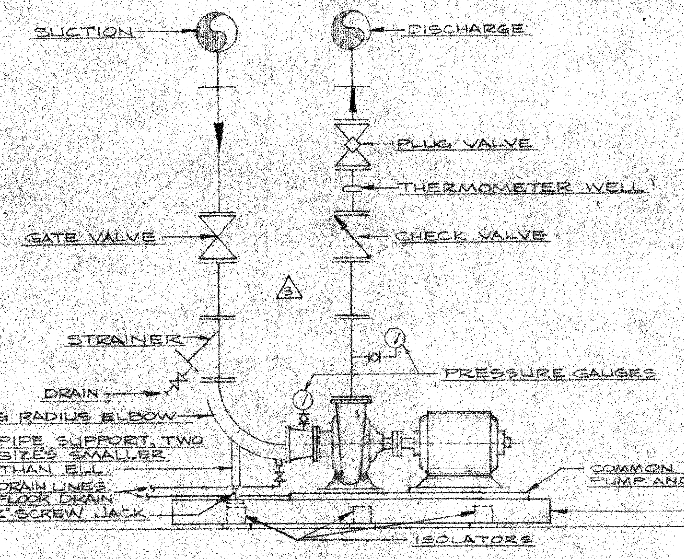
TYPICAL END SUCTION CENTRIFUGAL PUMP PIPING DIAGRAM NO SCALE
